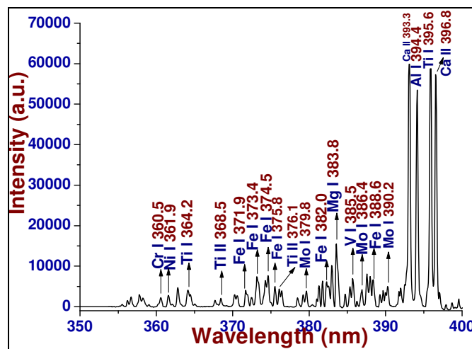
Fig. 2(a) : Recorded emission spectrum of Momordica Charantia excited by d c arc
