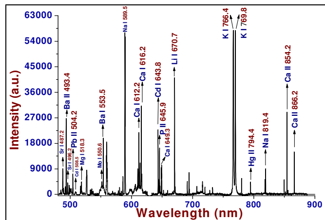
Fig. 2(c) : Recorded emission spectrum of Momordica Charantia excited by d c arc
