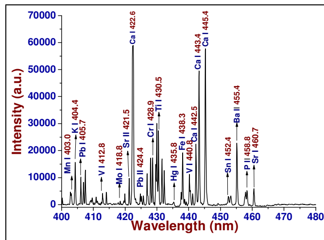
Fig. 2(b) : Recorded emission spectrum of Momordica Charantia excited by d c arc
