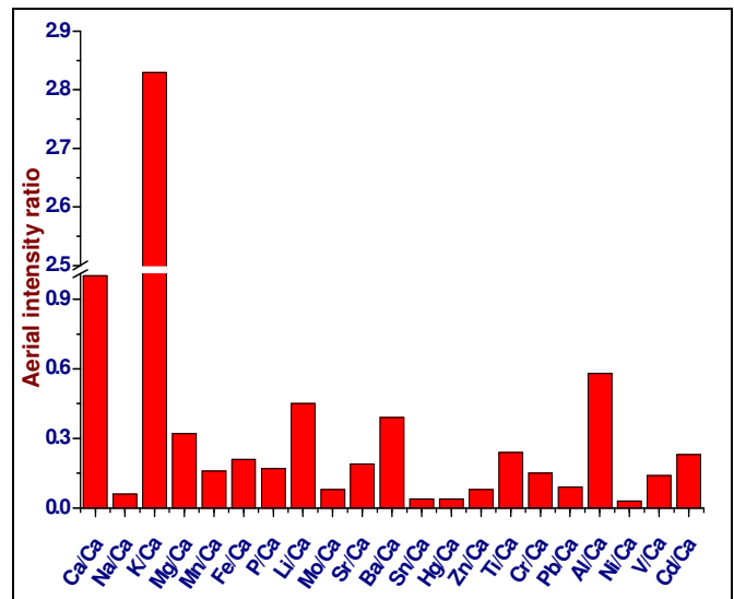
Fig. 3: Relative distribution of the detected elements in the Momordica Charantia
